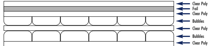
Seven layers; clear poly, foil, clear poly, bubbles, clear poly, bubbles and clear poly. Compression 6%.
