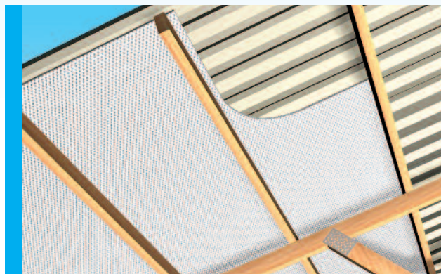
Roof / New* R-3.8 Heat Flow Down • R-3.5 Heat Flow Up
